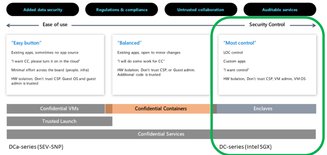
Confidential Computing Spectrum
